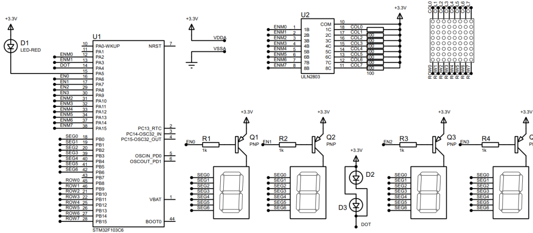
Figure 9: LED matrix is added to the simulation
