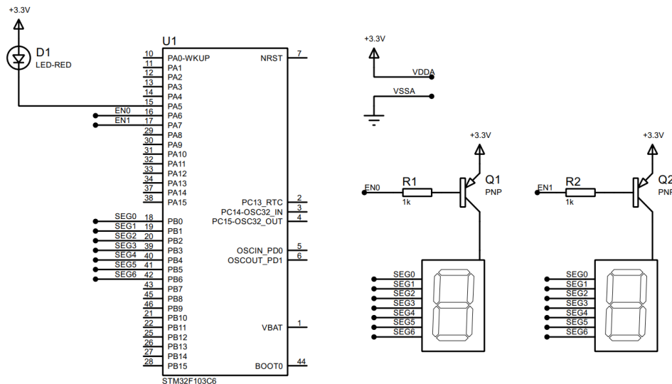
Figure 5: Simulation schematic in Proteus
